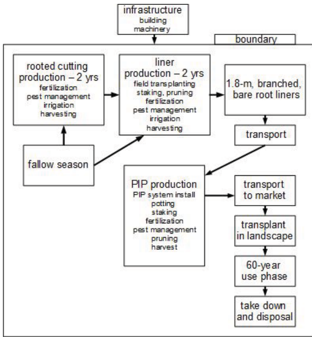
Fig. 1. Schematic of production system components of an Acer rubrum 'October Glory' in a #25 container from a pot-in-pot system.
